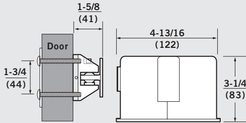
Overall Projection: 6-7/16" (164)
