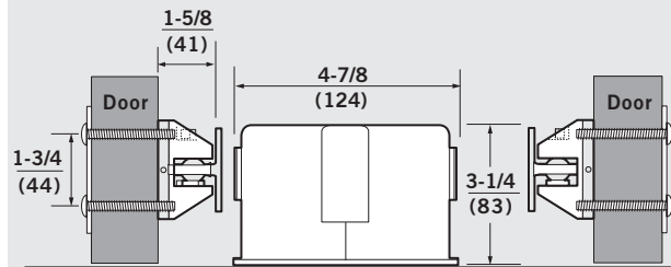
Overall Projection: 8-1/8" (206)
