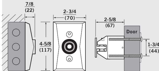
Overall Projection: 3-1/2" (89)
