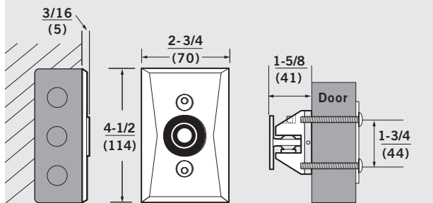
Overall Projection: 1-13/16" (46)
